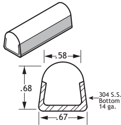
GRA-ROUND 10ft & 20ft Lengths
